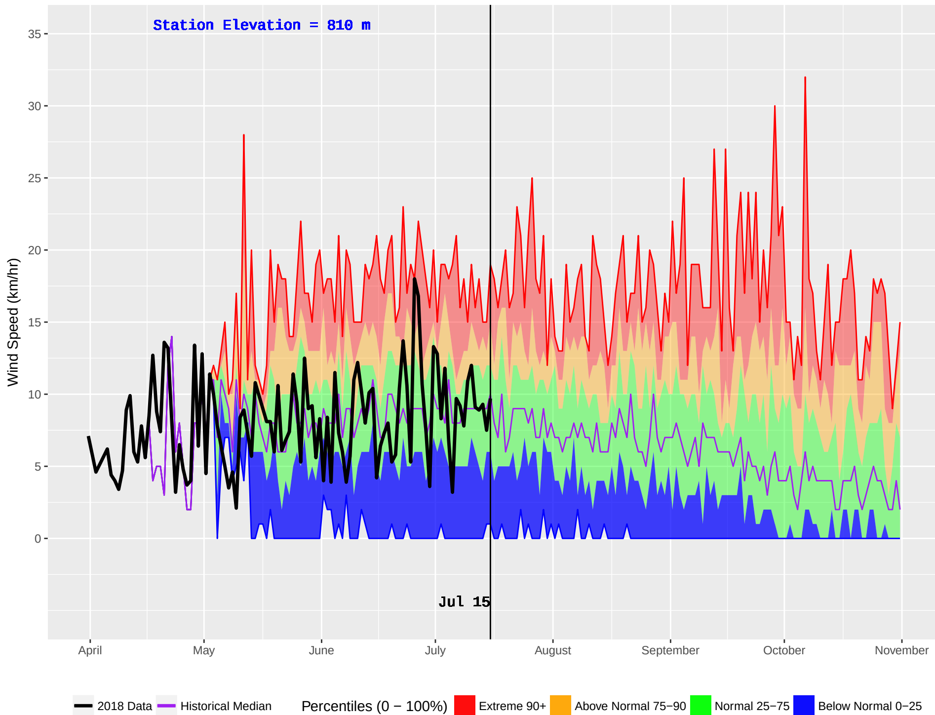
MCBRIDE LAKE (180) : Historical (1990–2016) and Current (2018) Daily Wind Speed
