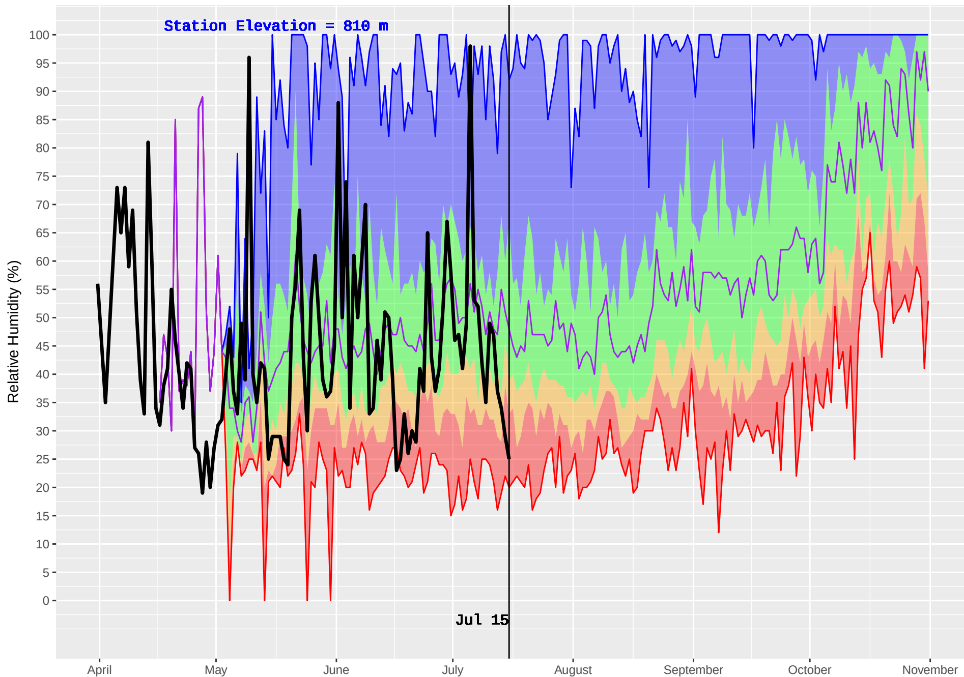
MCBRIDE LAKE (180) : Historical (1990–2016) and Current (2018) Daily Relative Humidity
